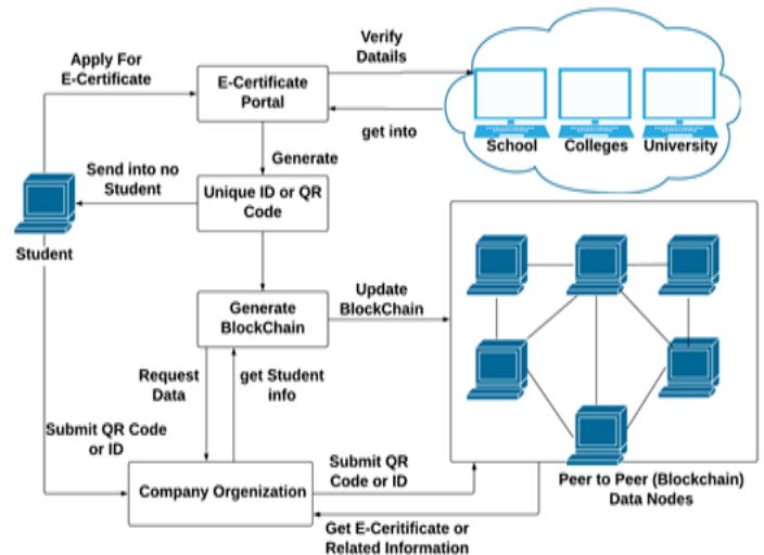
Figure 1 : System Architecture
