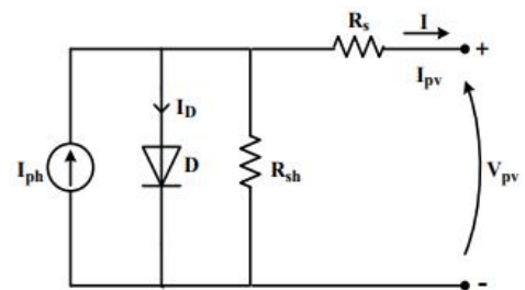
Fig. 1: The equivalent circuit of a PV array.
