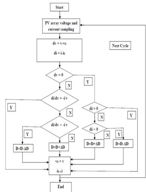
Fig. 2 Incremental conductance MPPT algorithm flow chart
