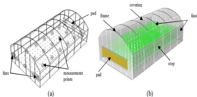
Fig. 1. (a) Wire-frame rendering of the greenhouse CAD model designed by Gambit® and experimental measurement points at level 1.2 m above ground. (b) 3D full scale simulation model of the experimental greenhouse with tomato crop.
