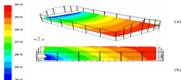
Fig. 3. Contours of air temperature a) plane surface 1.2 m above the ground and b) vertical surface in the middle of the greenhouse z=4.0 m (range 24–30°C).
