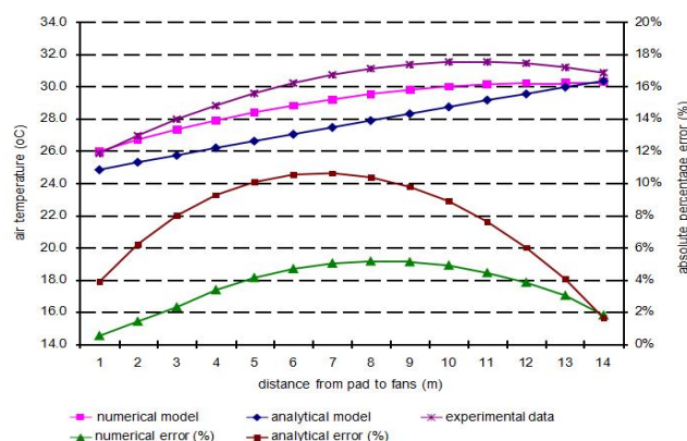
Fig. 2. XY scattering of air temperature inside the greenhouse. Comparison of the average values obtained by the numerical and analytical model with experimental data.
