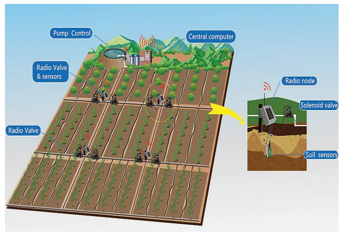
Figure 2: Precision agriculture
